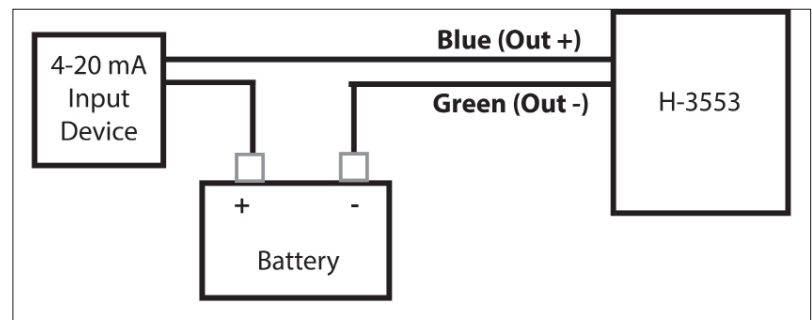
Figure 4-1: Typical H-3553T 4-20 mA Output Setup
